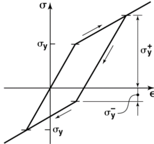
Figure 2-36 Bauschinger Effect for a Linear Strain-Hardening Curve
