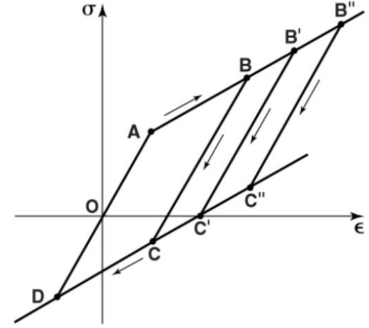
Figure 2-37 Bauschinger Effect for a Linear Strain-Hardening Curve with Multiple Load-Unload Cycles
