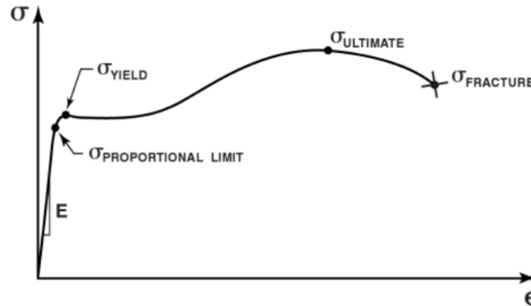
Figure 1-3 Stress-Strain Behavior of Mild Steel
