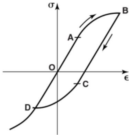
Figure 2-35 Bauschinger Effect for a General Linear-Nonlinear Curve
